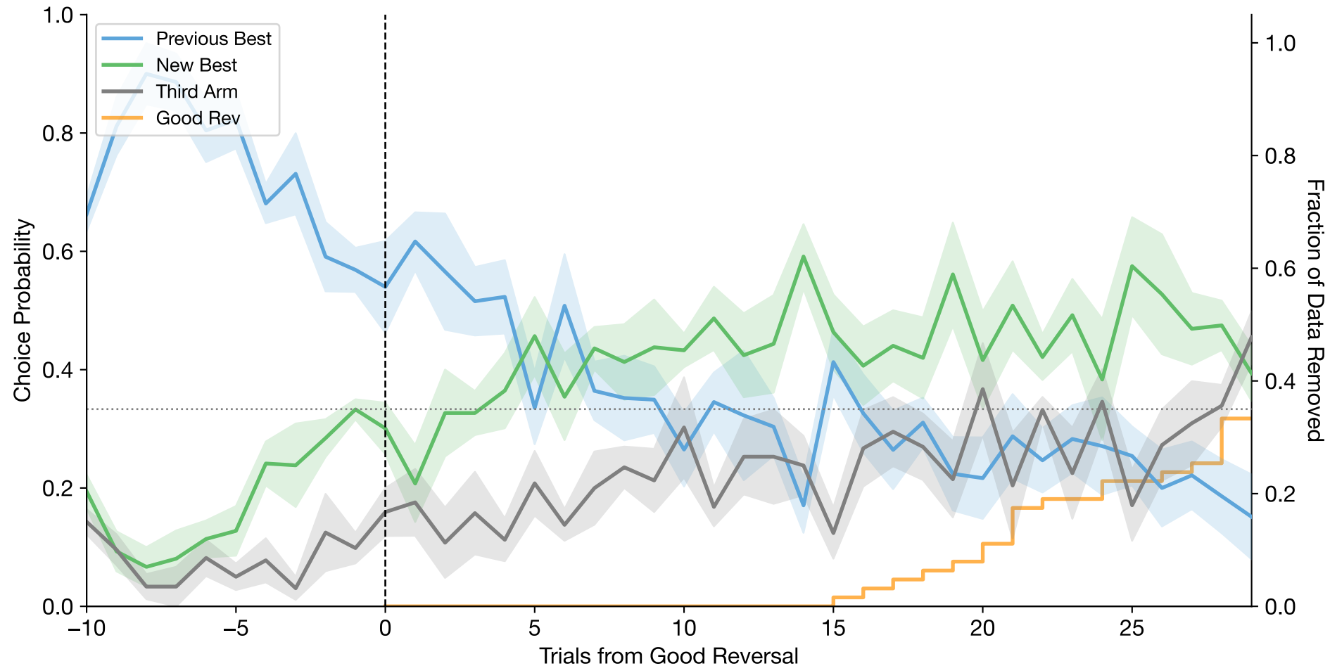
Good Reversal-Aligned Choices (mean \pm se across subjects | n=6 subjects, n=63 reversals)
